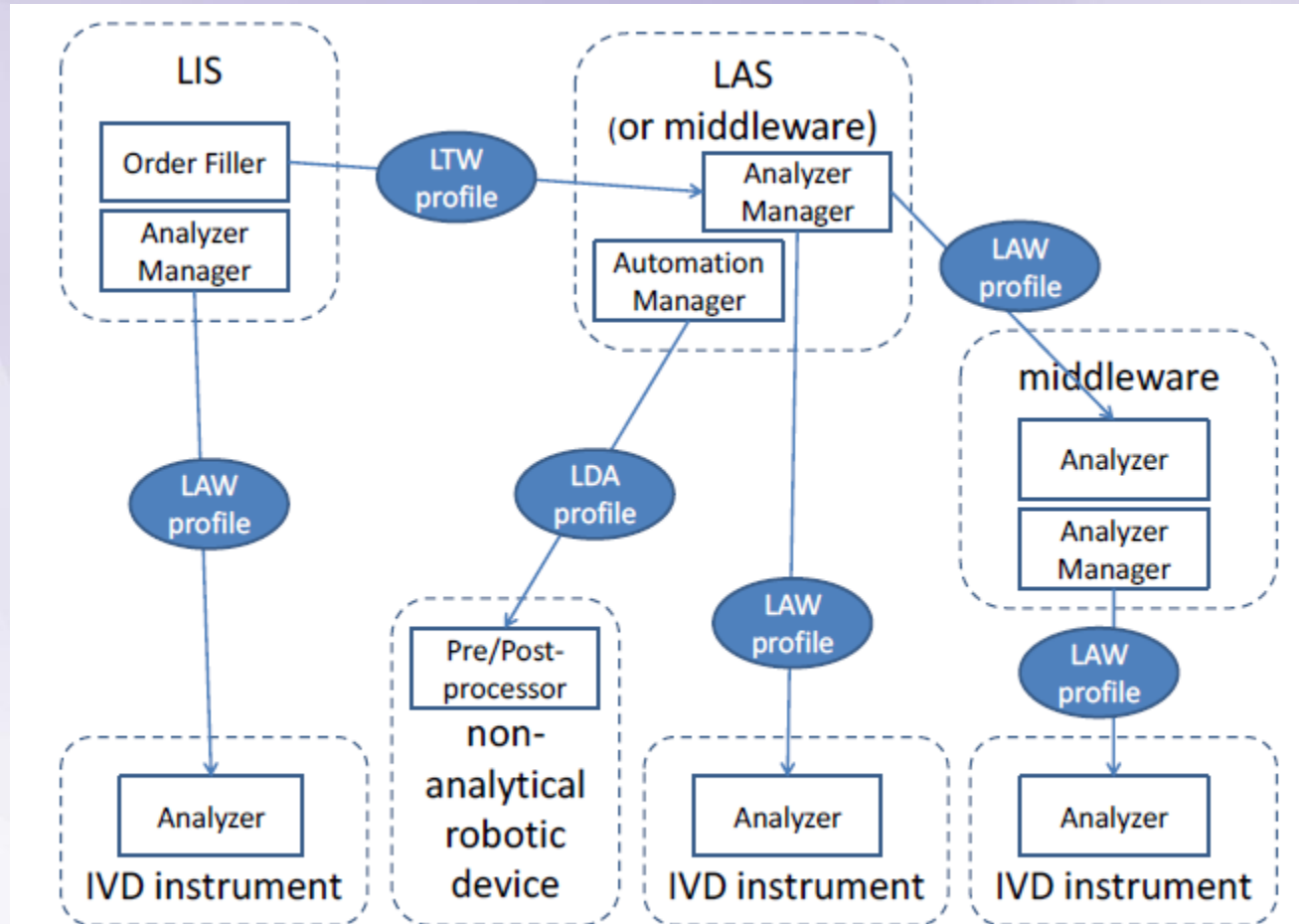
Figure X.3-1: Interconnection of systems and mapping to profile's actors
